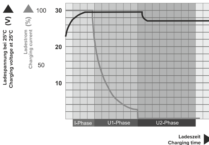
Ladekennlinie Charging characteristic
