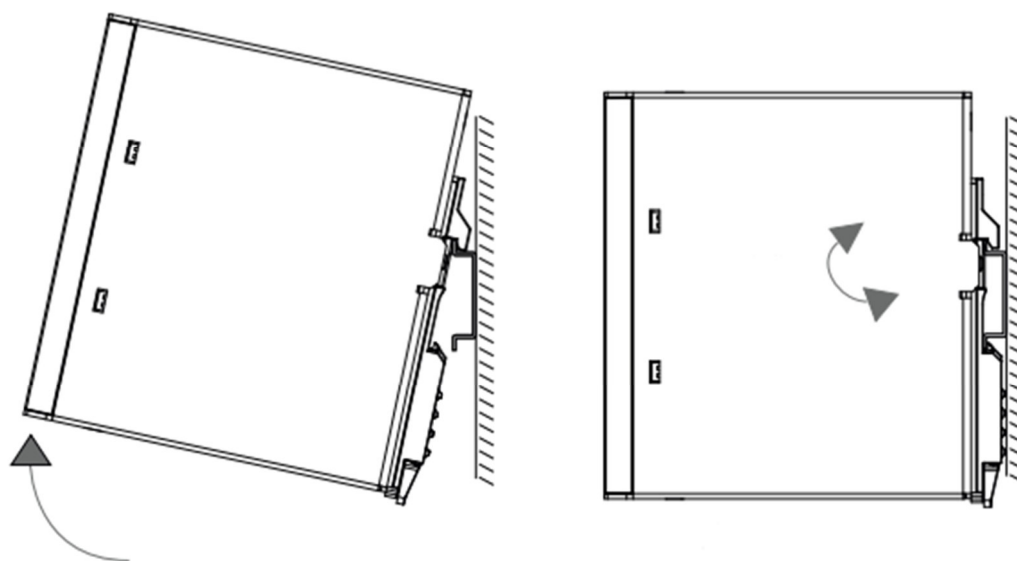
Figure 5: Assembly
