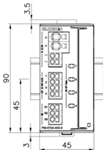
Dimensions 4/2- channel modules
